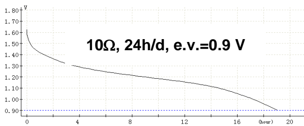
Chart 1. Discharge diagram
